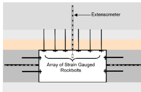
A TYPICAL ROOFBOLTED ROADWAY MONITORING STATION
